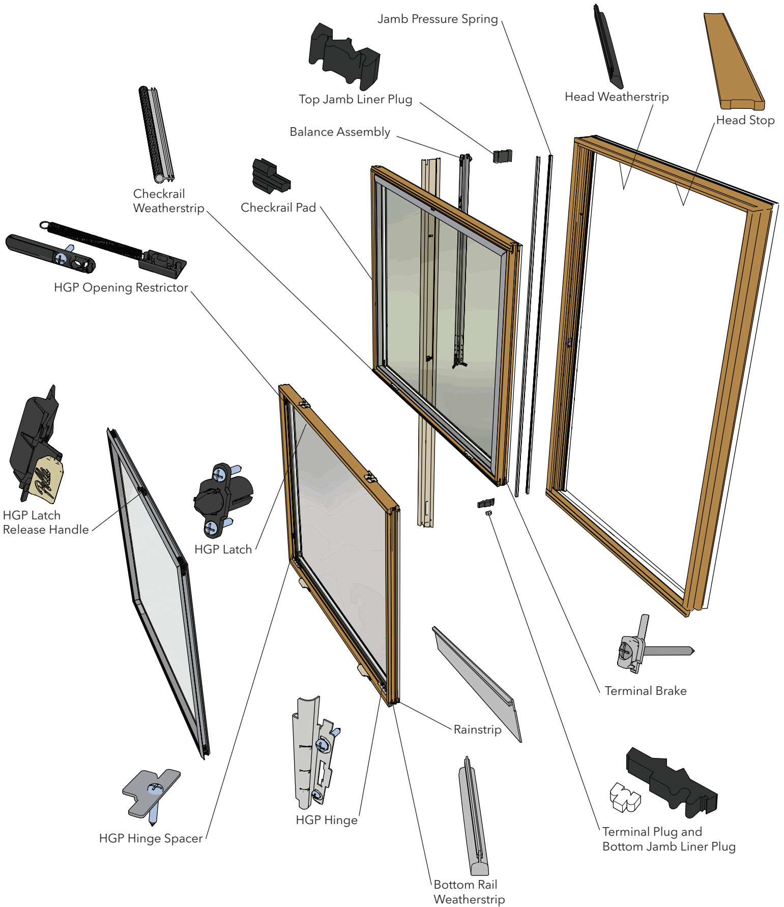
Interior View
